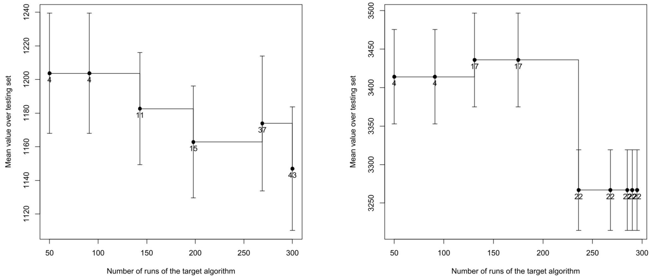
Figure 2: Graphical representation of SA output for instances of size 50 (left) and 100 (right).
